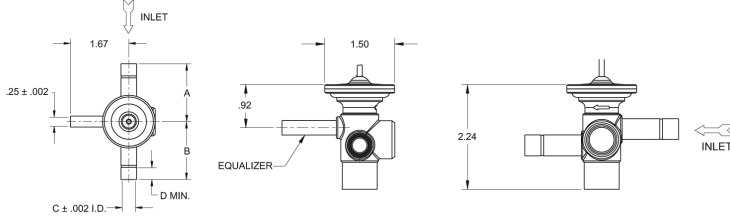
Non-Adjustable - ODF Connections with 1/4 ODF Equalizer Shown
